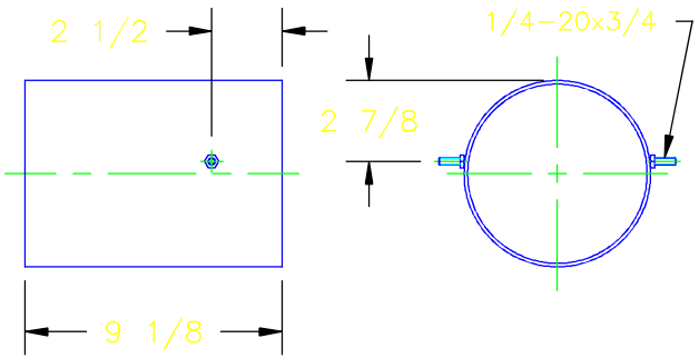
DISCHARGE TUBE MATL: 1/8x6 PIPE
